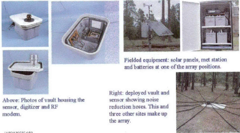
Figure 17: A prototype infrasound array, from [24]
