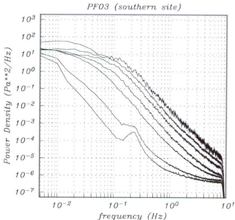
Figure 13: This figure shows the acoustical energy per unit bandwidth, in \text{Pa}^2/\text{Hz} , parameterized by wind speed. For appreciable wind speeds the energy per unit bandwidth falls at 1/f^3 . At low wind speeds the ‘microbarom’ of geophysical origin is clearly visible. Note also the sensor noise floor at 3 \times 10^{-7} . From [34].
